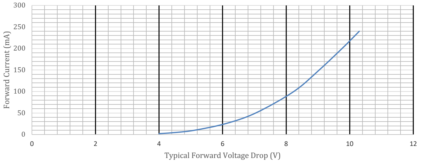
Forward Current vs. Typical Forward Voltage Drop XGF08
