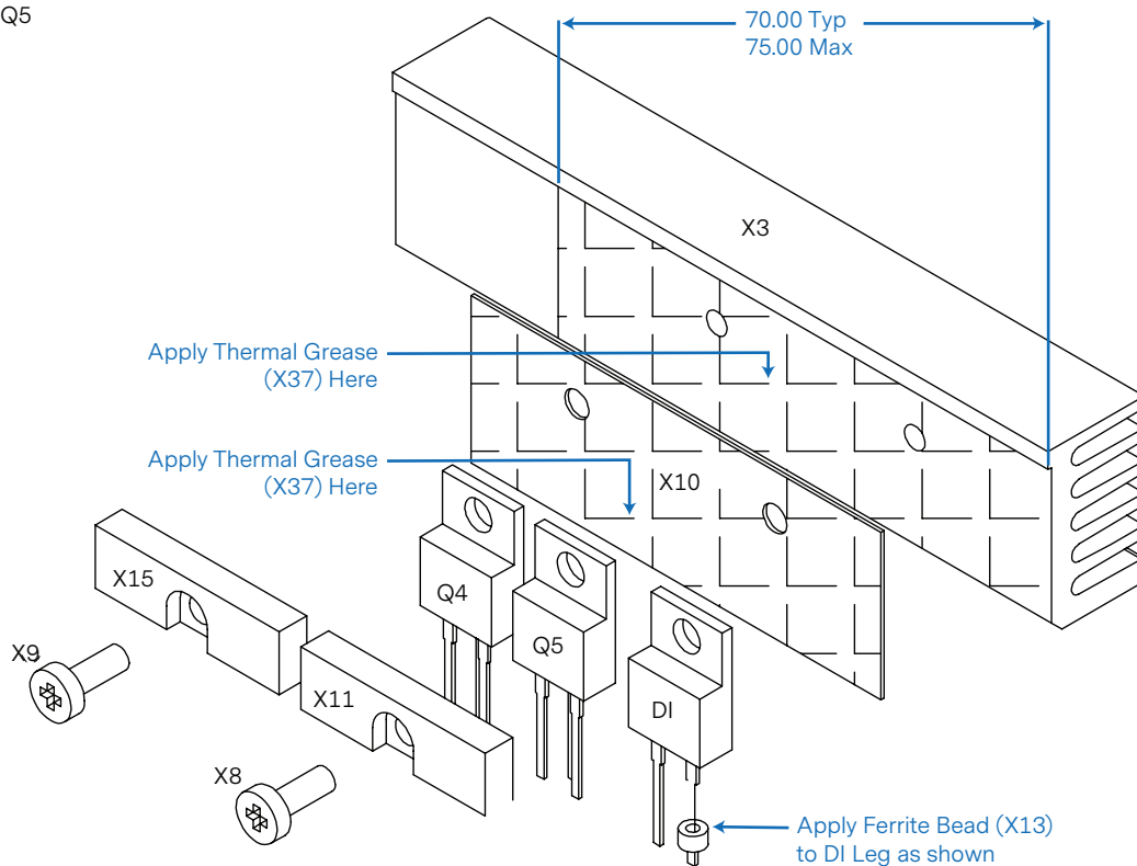
Figure 2: A combination of conduction and convection cooling provide effective thermal management
