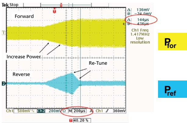
Above, reflected power is minimized ~150 μsec after plasma power set point change.
